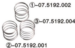
CWN-M458 漲力器彈簧 IRO
