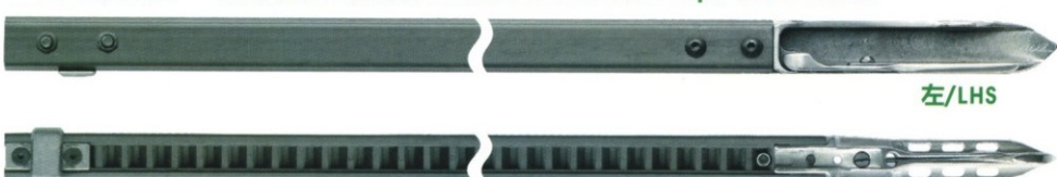
CWN-VD003 范德维尔丝绒剑杆 NT.OLD1-Carbon Tape With Head
